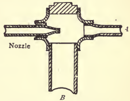
FIG. 34.—APPLIANCE FOR CLEANING SIPHON-SUMP.
